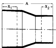
Concentric Reducer
